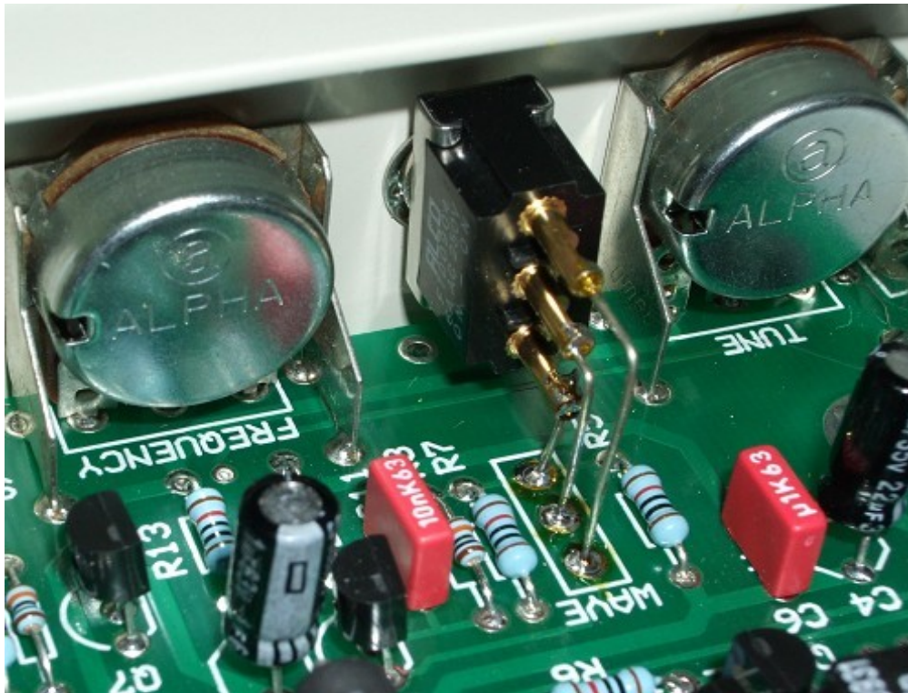
This is a TM3030 issue 1 PCB that uses a panel mounted switch. I wanted to use this type of switch because the panel itself was too thick to use the normal PCB mounted switches we use. Note the use of preformed tinned solid core wire to make the connections.
