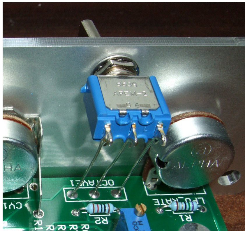
This is the switch on a VCO Controller module. The issue 2 SVCO PCBs should be wired similarly with the each tang connected to the solder pad directly below it.
