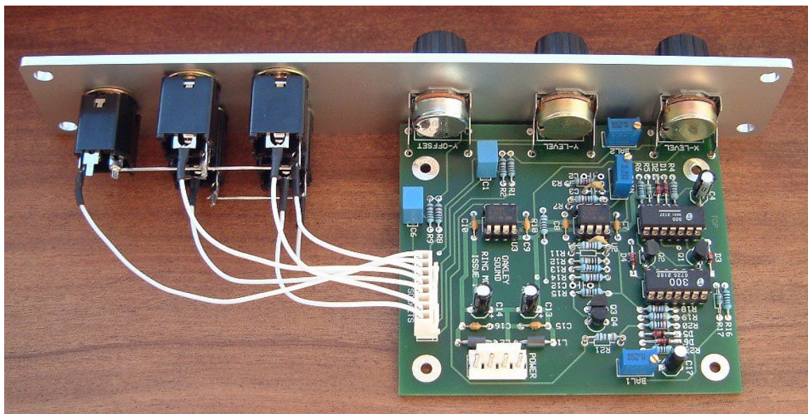
This is the prototype issue 1 RM4014 Ring Modulator module behind a natural finish 1U wide MOTM format Schaeffer panel.
